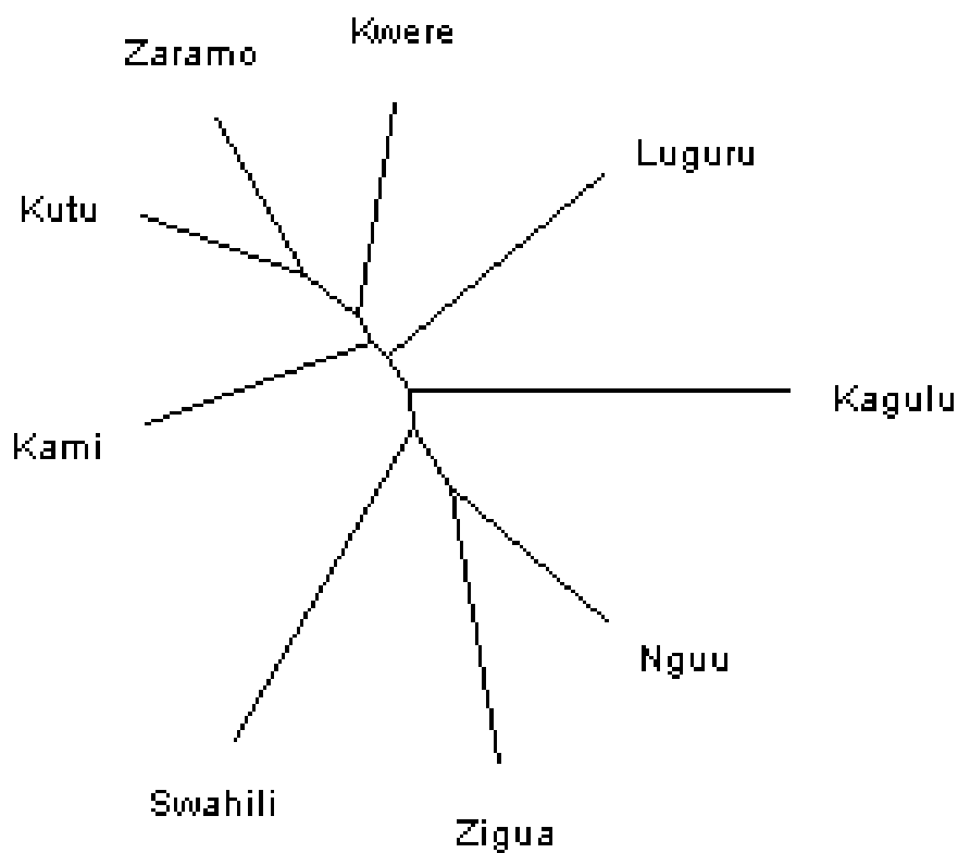
Figure 4. A neighbour-joining tree based on the lexical distance matrix of Table 8.
