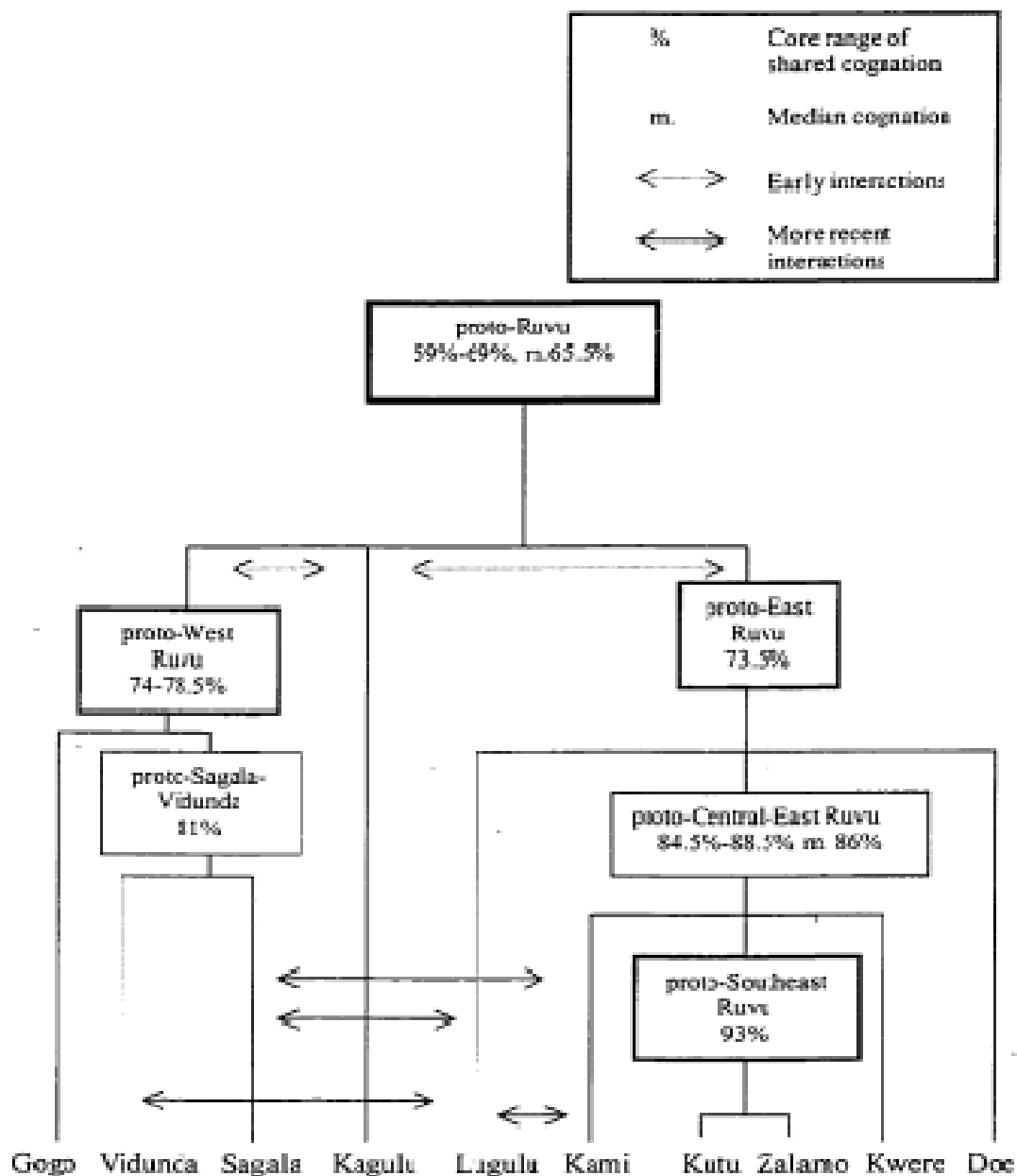
Figure 3. Gonzales' (2002: 34) classification of the Ruvu languages.
